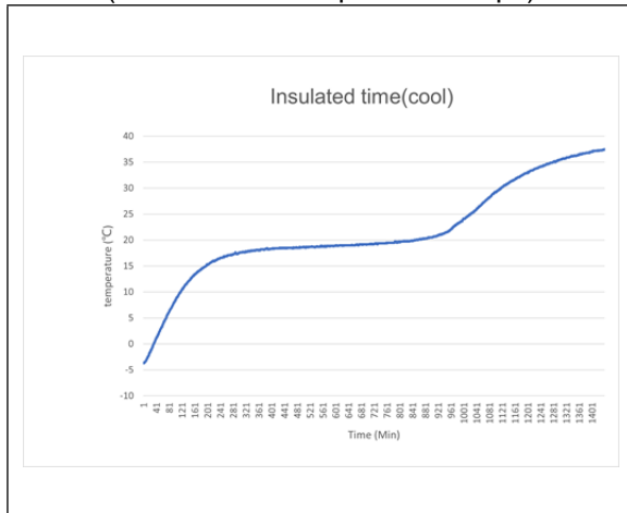
Insulation performance curve chart (40°C Thermos cup + 8 ice strips)
