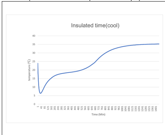
Insulation performance curve chart (35°C Thermos cup + 4 ice strips)
