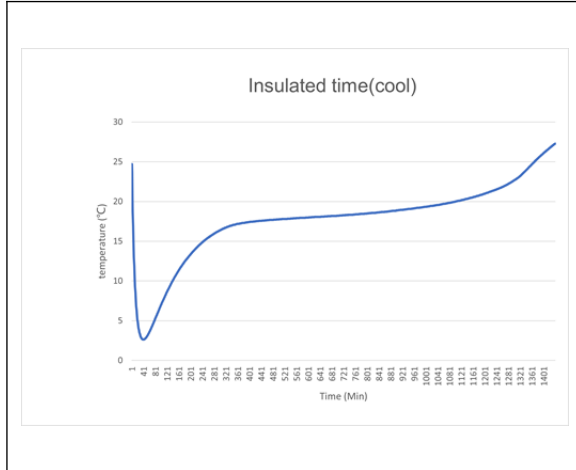
Insulation performance curve chart (40°C Thermos cup + 2 ice strips)
