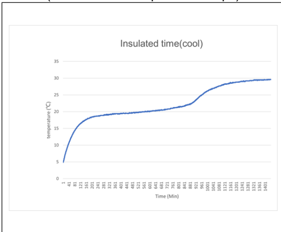
Insulation performance curve chart (30°C Thermos cup + 4 ice strips)
