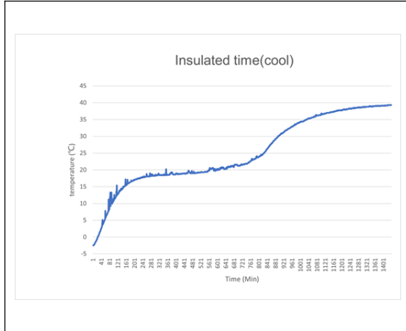
Insulation performance curve chart (40°C Thermos cup + 10 ice strips)
