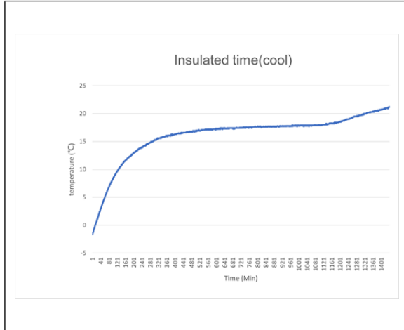
Insulation performance curve chart (35°C Thermos cup + 2 ice strips)
