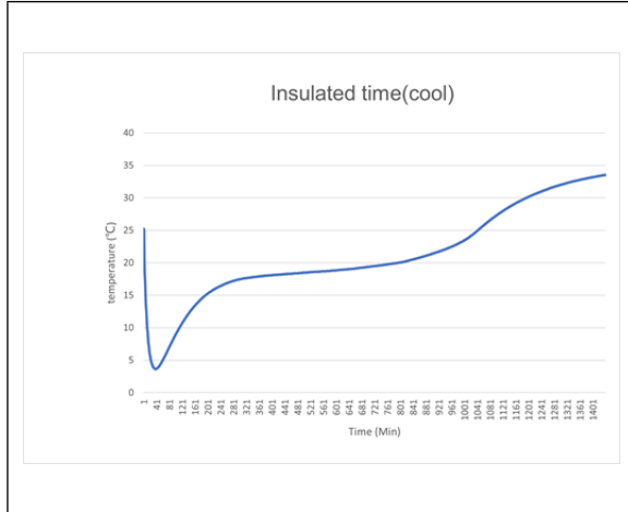
Insulation performance curve chart (35°C Thermos cup + 10 ice strips)
