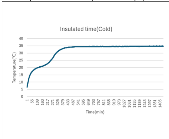
Insulation performance curve chart (35°C Thermos cup + 1 ice strips)
