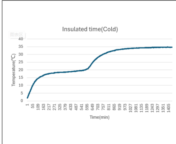
Insulation performance curve chart (35°C Thermos cup + 5 ice strips)
