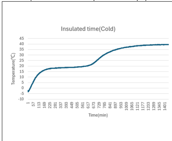
Insulation performance curve chart (40°C Thermos cup + 4 ice strips)
