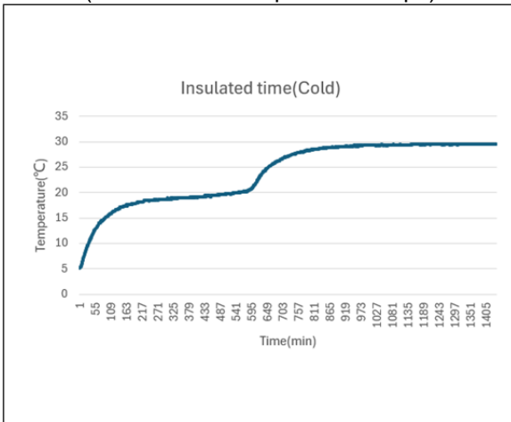
Insulation performance curve chart (30°C Thermos cup + 2 ice strips)
