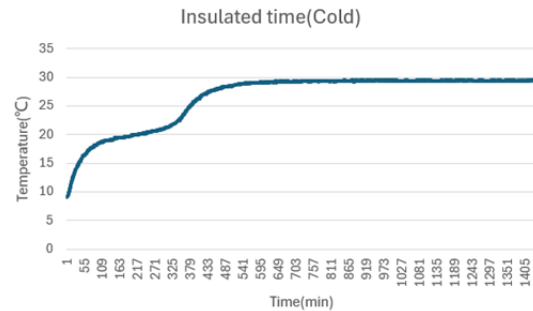
Insulation performance curve chart (30°C Thermos cup + 3 ice strips)
