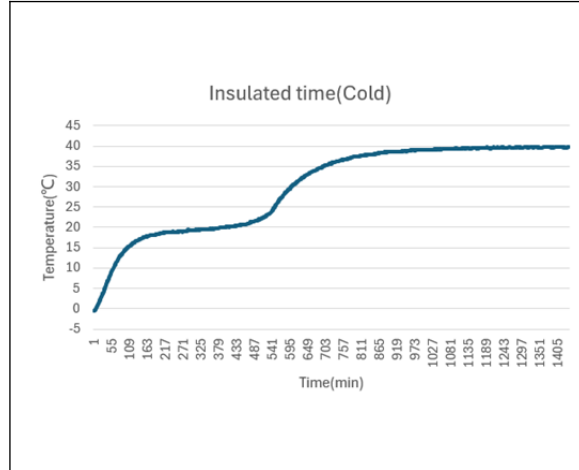
Insulation performance curve chart (40°C Thermos cup + 5 ice strips)
