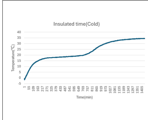
Insulation performance curve chart (40°C Thermos cup + 1 ice strips)
